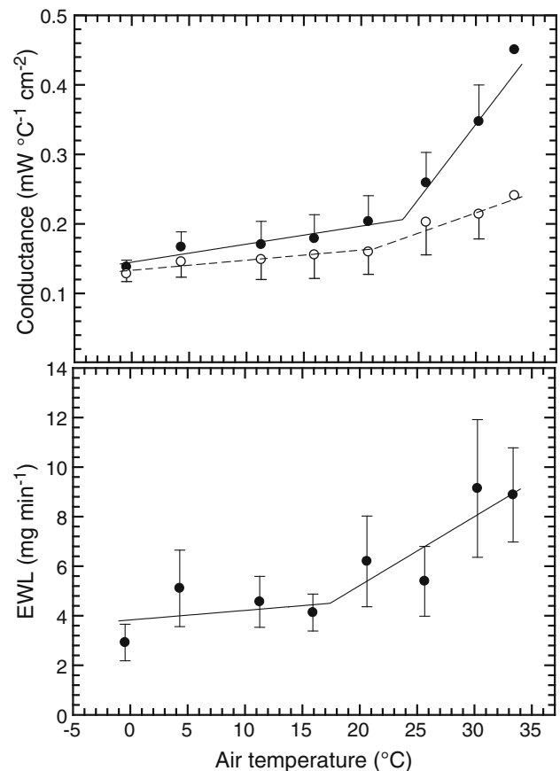
Fig. 2 Relationships among total thermal conductance (top panel; filled symbols), dry heat transfer coefficient (top panel; clear symbols) and evaporative water loss (EWL; bottom panel) and air temperature ( T_a ) in African Green Pigeons ( Treron calvus ) measured under laboratory conditions. Error bars indicate standard deviations. The solid and dashed lines represent broken-stick regression models fitted to the raw data, not the mean values plotted here. Samples sizes for EWL varied from 6 to 10 per T_a , but intermittent PIT tag reception resulted in incomplete body temperature records for some birds, and sample sizes of conductance values thus varied from 1 to 7
